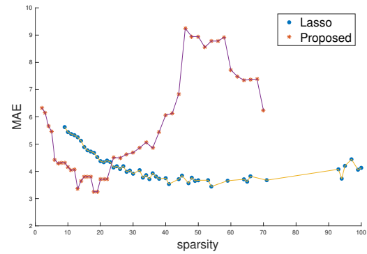
Fig. 5. MAE of Proposed scheme and Lasso with different sparsity
