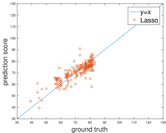
Fig. 4. Lasso score correlation
