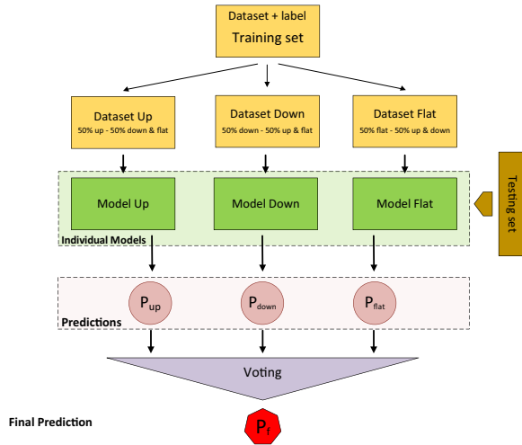
Fig. 2: Ensemble Strategy. Training m models to detect M activities. In voting block, the best prediction gets selected.
