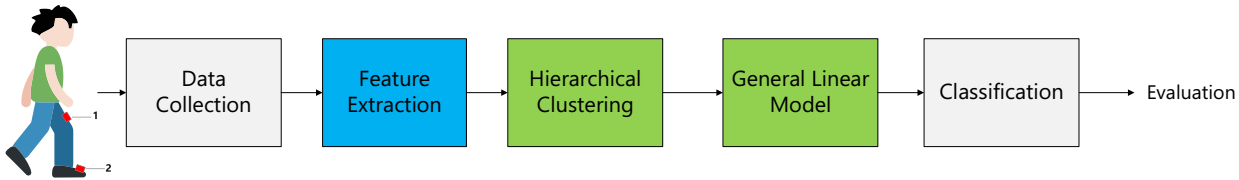
Fig. 1: Main approach for Human Activity Recognition. Two red squares show sensor positions on the thigh and foot of the subject. The green blocks show the feature selection phase.
