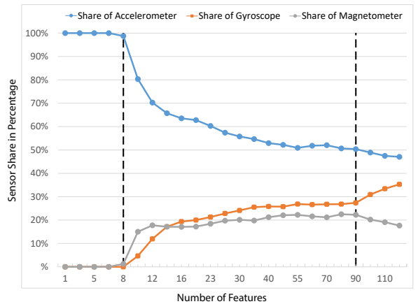
Fig. 3: contribution of three sensors over different sizes of featureset
